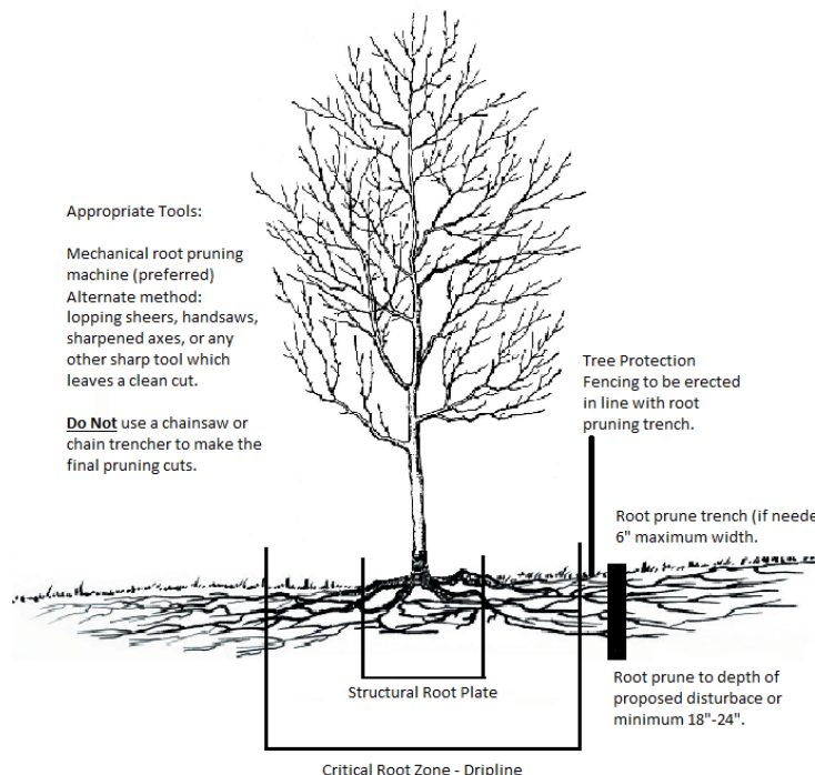
ROOT PRUNING DETAIL
