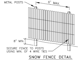
SNOW FENCE DETAIL
