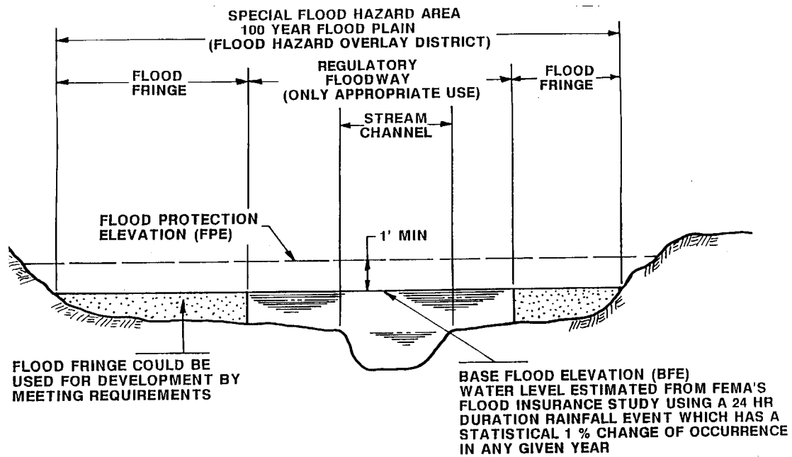
TYPICAL FLOODPLAIN CROSS-SECTION
