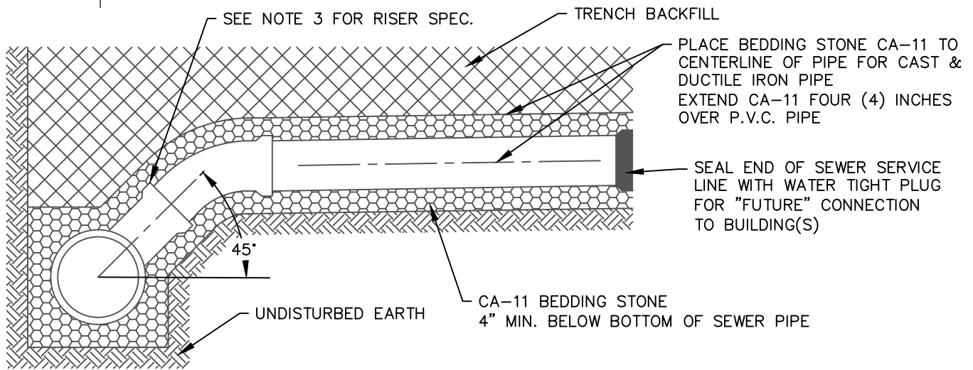
ELEVATION VIEW
